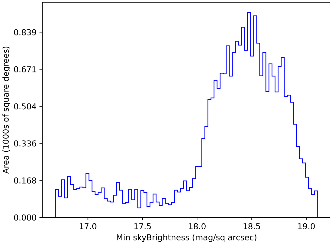
ddf_loaded_fl15_v3.4_10yrs Yr 1 z band: Min skyBrightness
