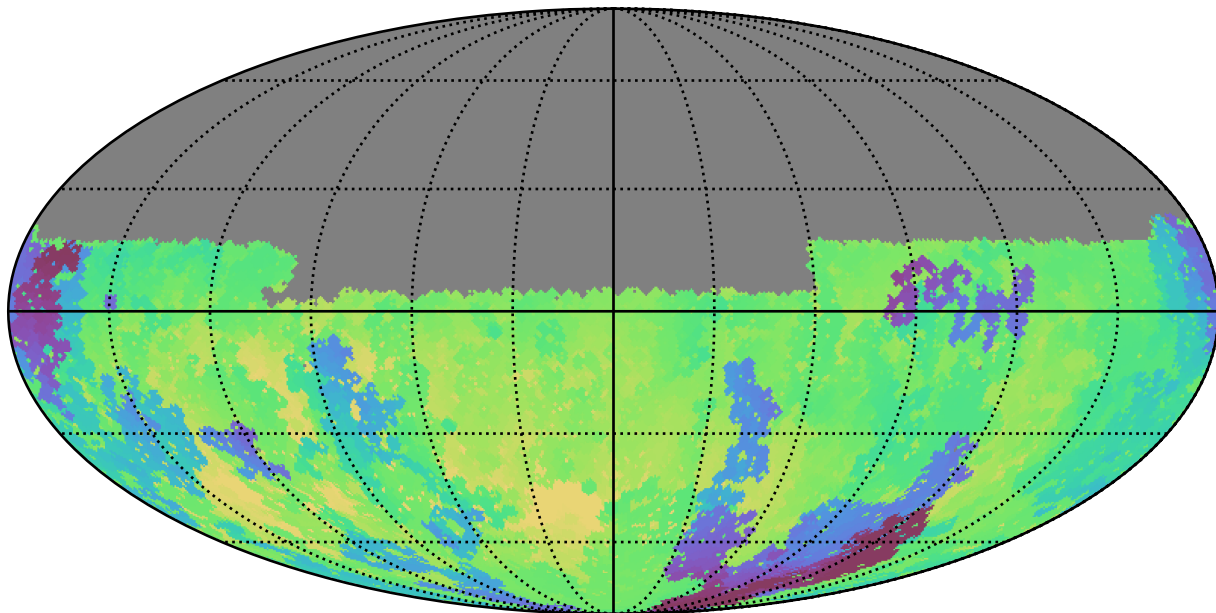
ddf_loaded_fl15_v3.4_10yrs Yr 1 u band: Min skyBrightness
