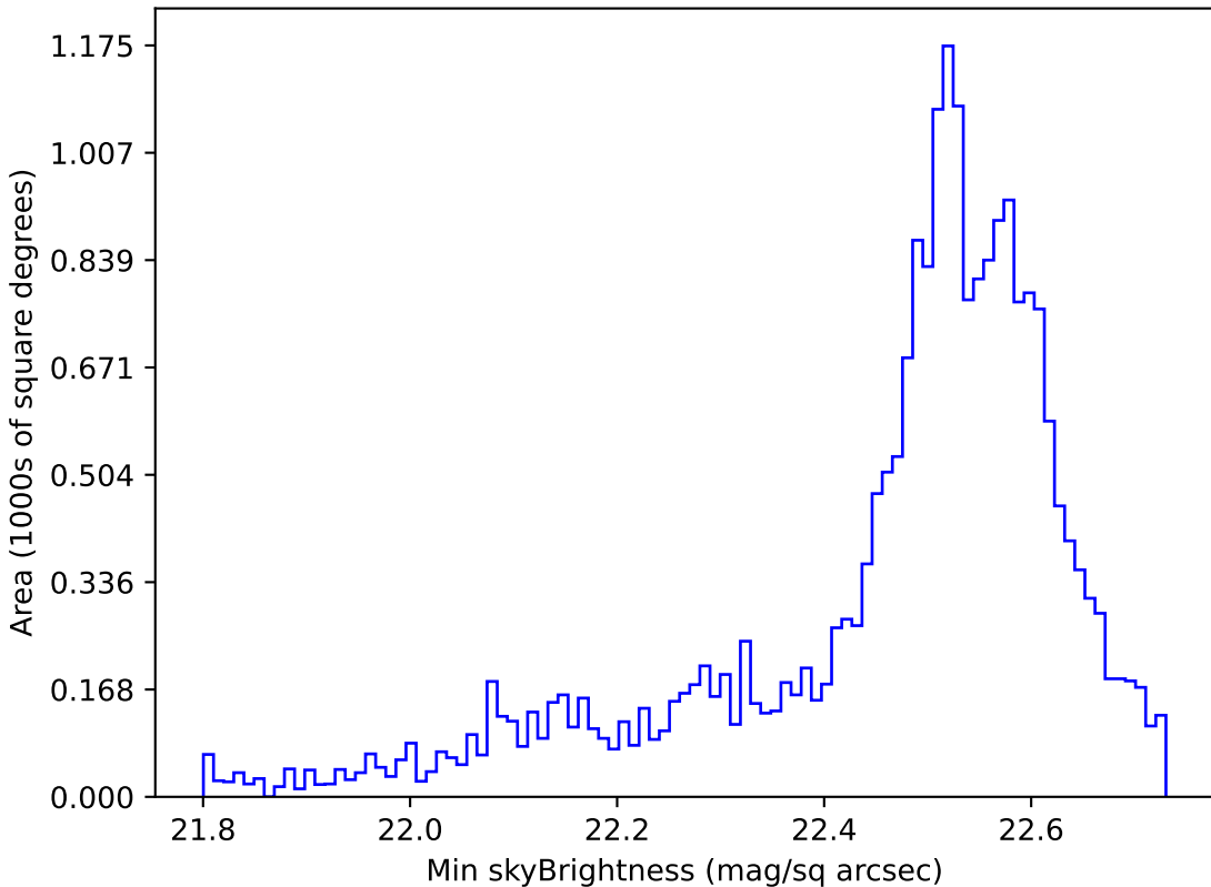
ddf_loaded_fl15_v3.4_10yrs Yr 1 u band: Min skyBrightness
