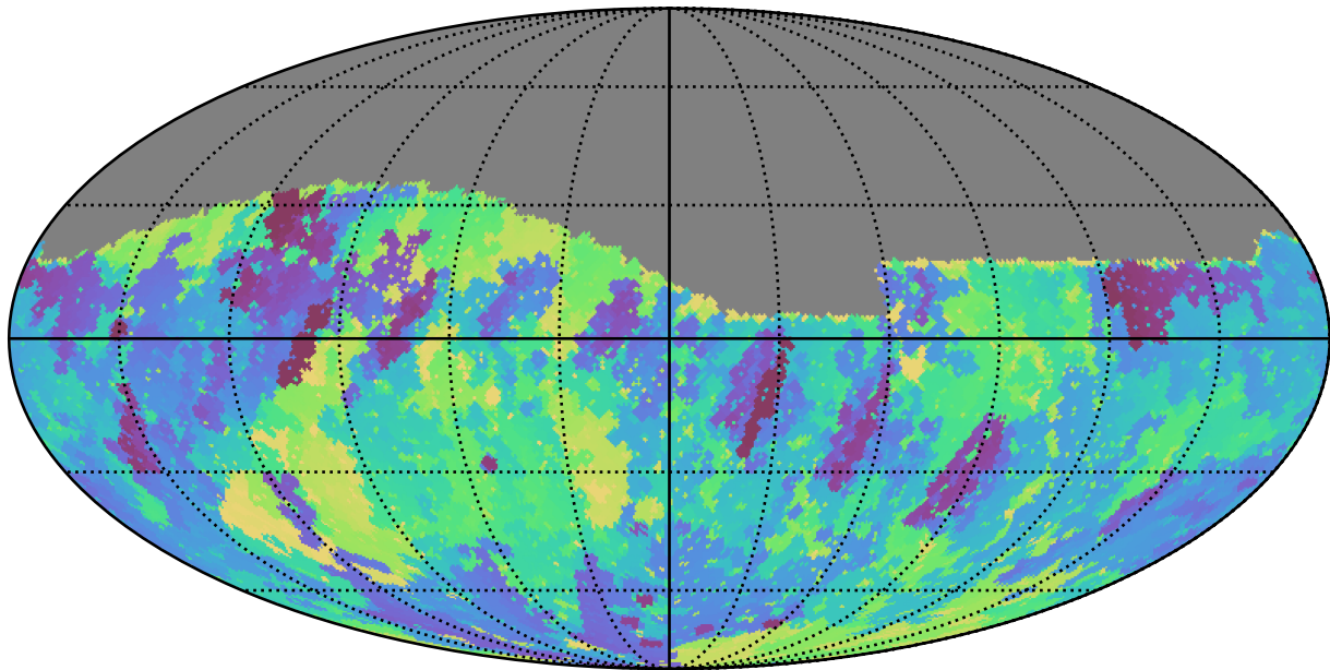
ddf_loaded_fl15_v3.4_10yrs Yr 1 r band: Min skyBrightness
