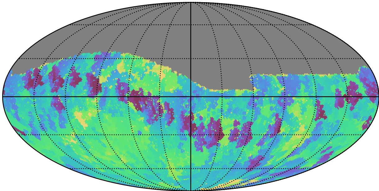
ddf_loaded_fl15_v3.4_10yrs Yr 1 i band: Min skyBrightness
