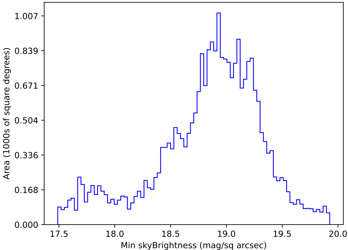
ddf_loaded_fl15_v3.4_10yrs Yr 1 i band: Min skyBrightness
