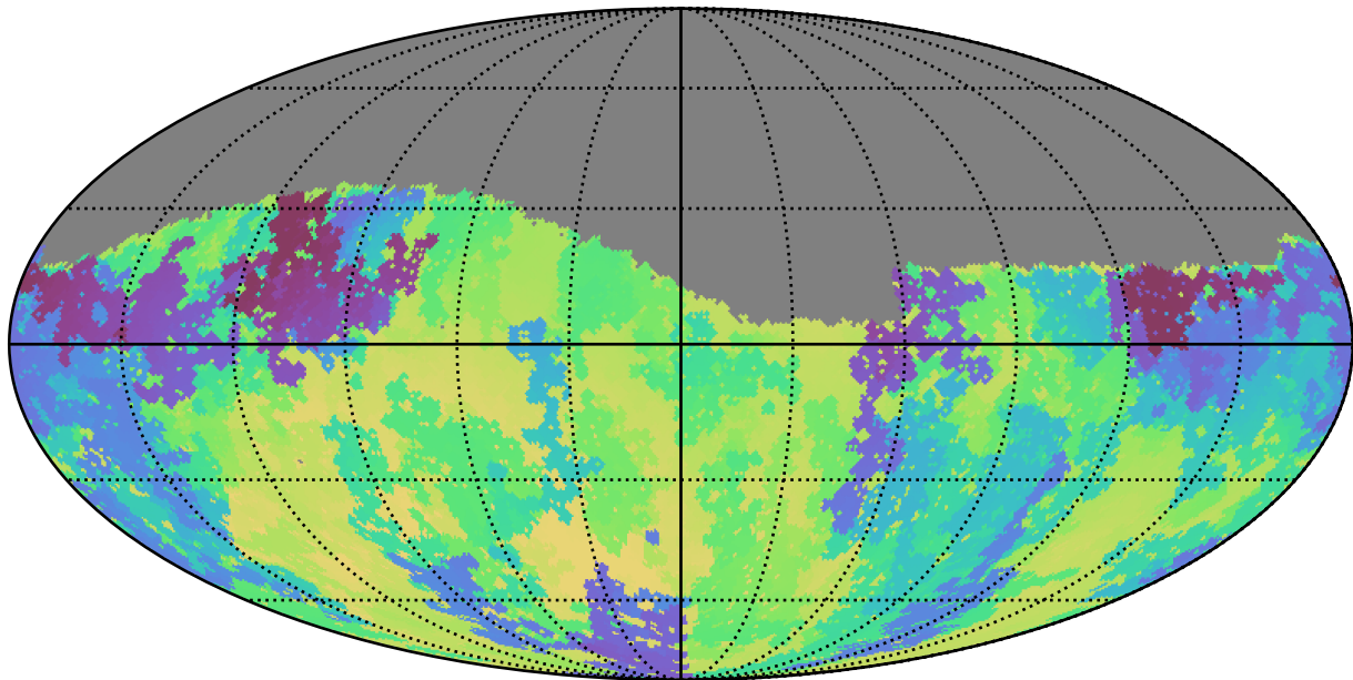
ddf_loaded_fl15_v3.4_10yrs Yr 1 g band: Min skyBrightness
