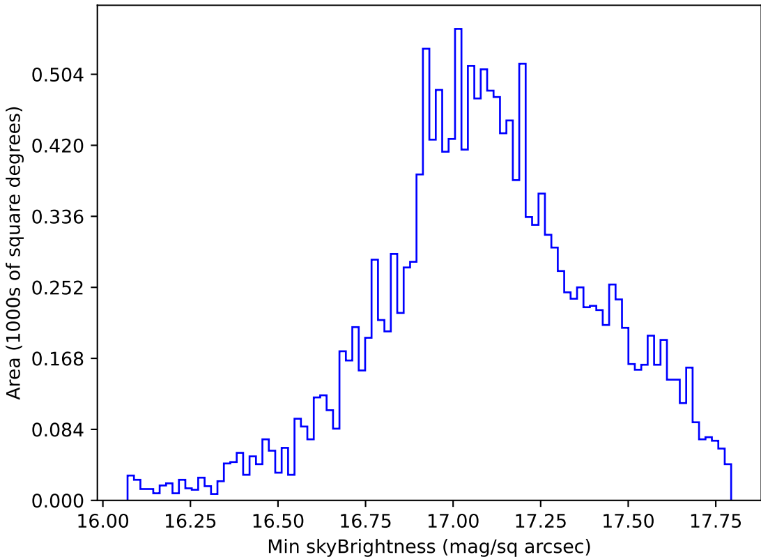
ddf_loaded_fl15_v3.4_10yrs WFD y band: Min skyBrightness
