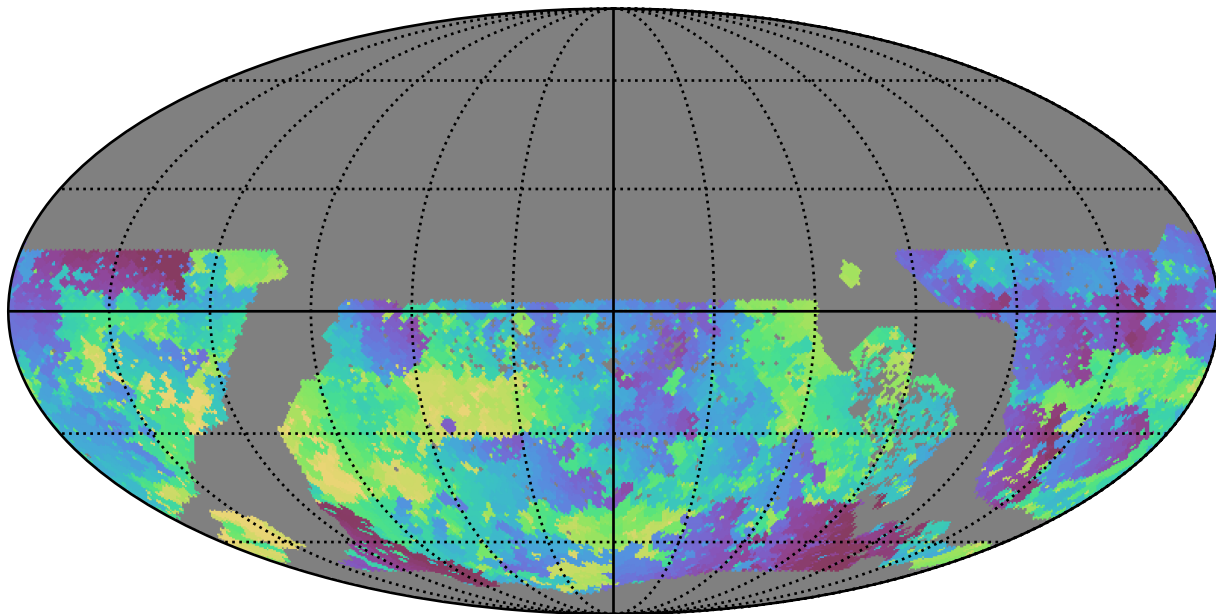
ddf_loaded_fl15_v3.4_10yrs WFD u band: Min skyBrightness
