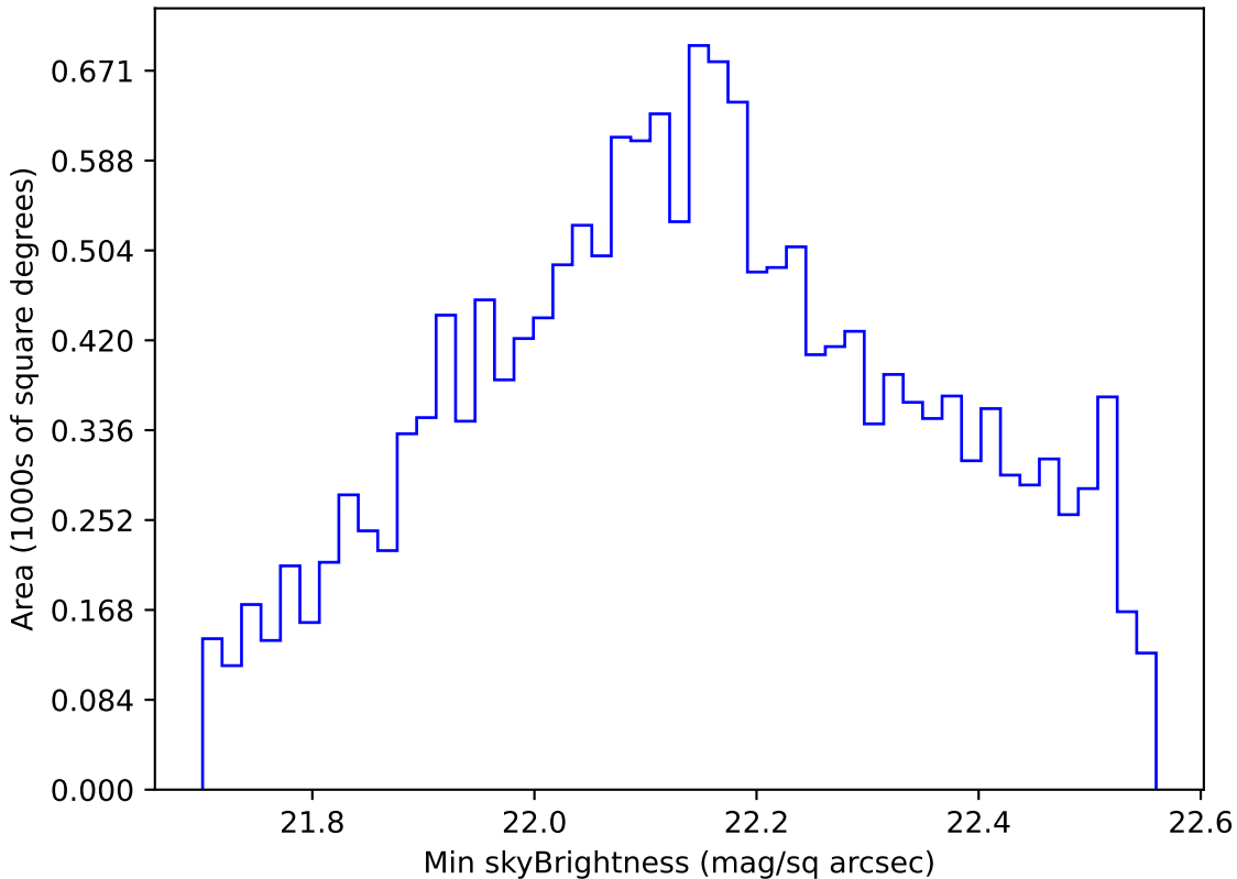
ddf_loaded_fl15_v3.4_10yrs WFD u band: Min skyBrightness
