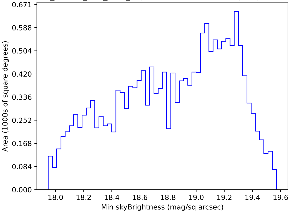
ddf_loaded_fl15_v3.4_10yrs WFD r band: Min skyBrightness
