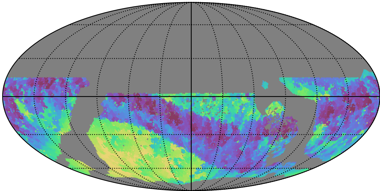
ddf_loaded_fl15_v3.4_10yrs WFD i band: Min skyBrightness
