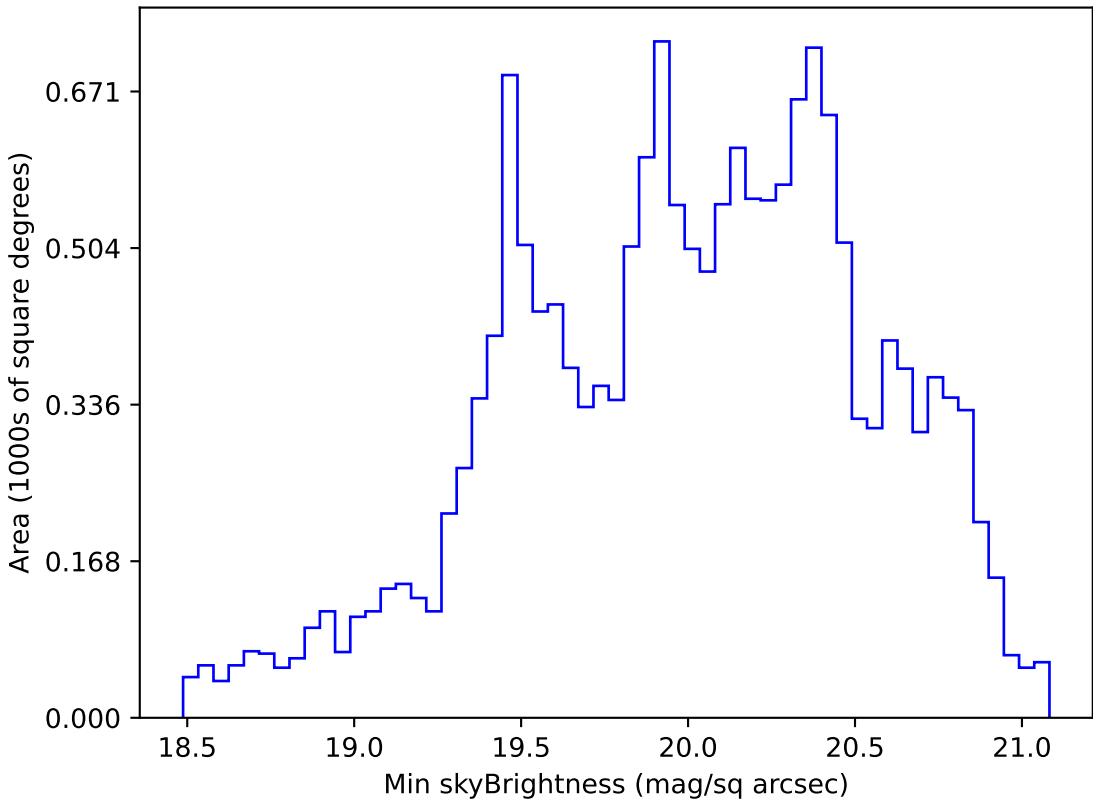
ddf_loaded_fl15_v3.4_10yrs WFD g band: Min skyBrightness
