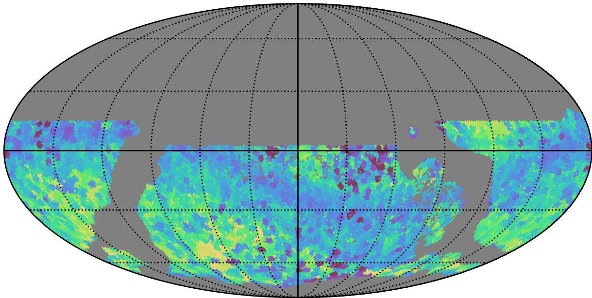
ddf_loaded_fl15_v3.4_10yrs WFD all bands: Min skyBrightness
