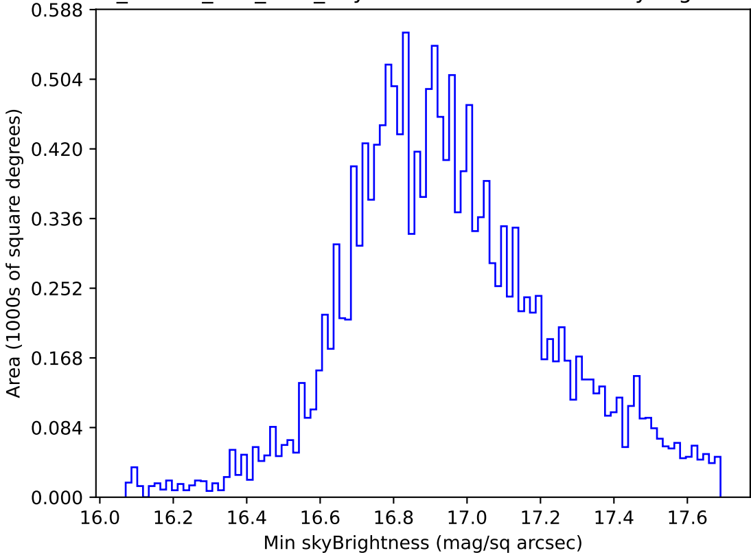
ddf_loaded_fl15_v3.4_10yrs WFD all bands: Min skyBrightness
