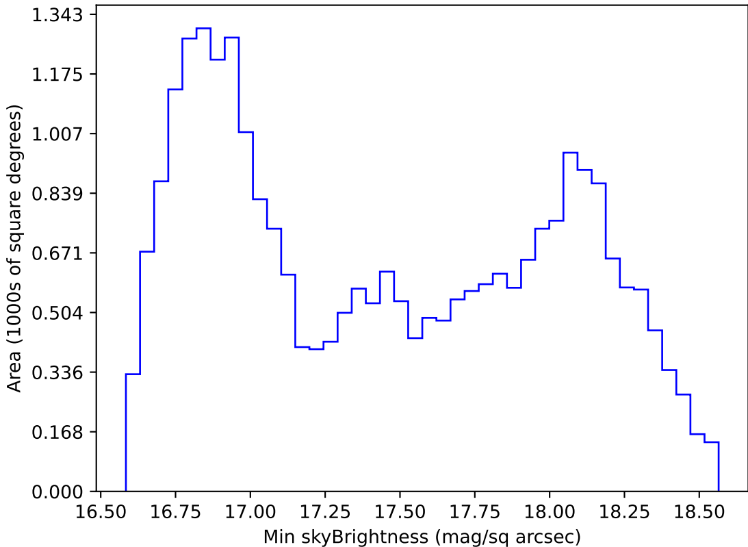
ddf_loaded_fl15_v3.4_10yrs All sky z band: Min skyBrightness
