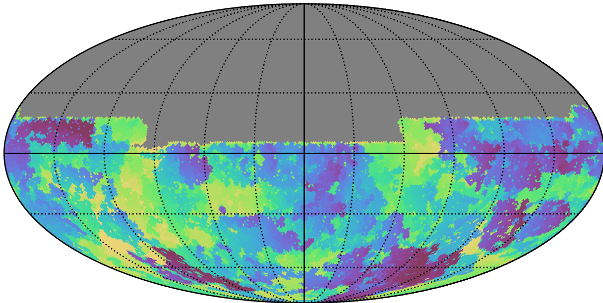
ddf_loaded_fl15_v3.4_10yrs All sky u band: Min skyBrightness
