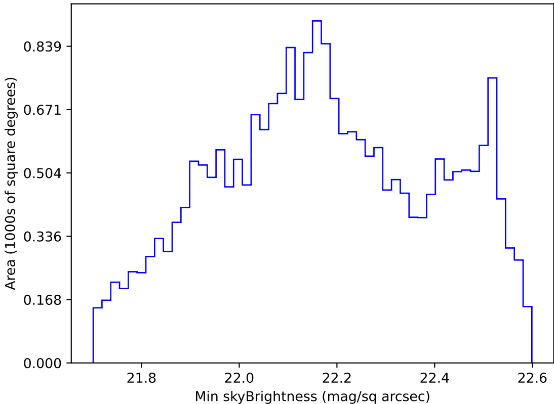
ddf_loaded_fl15_v3.4_10yrs All sky u band: Min skyBrightness
