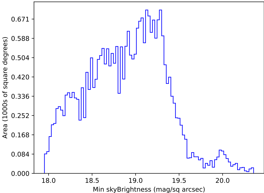
ddf_loaded_fl15_v3.4_10yrs All sky r band: Min skyBrightness
