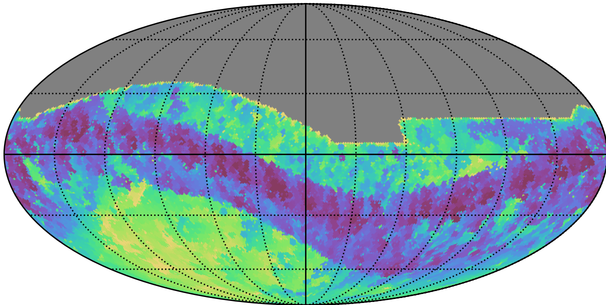
ddf_loaded_fl15_v3.4_10yrs All sky i band: Min skyBrightness
