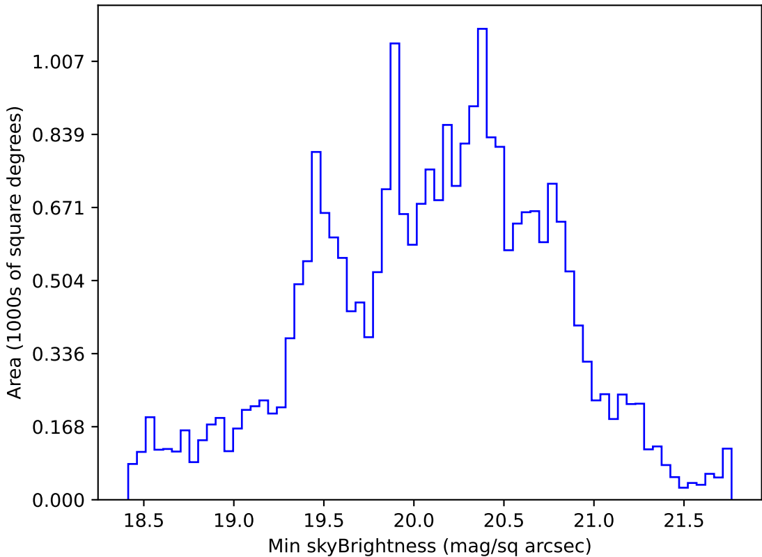
ddf_loaded_fl15_v3.4_10yrs All sky g band: Min skyBrightness
