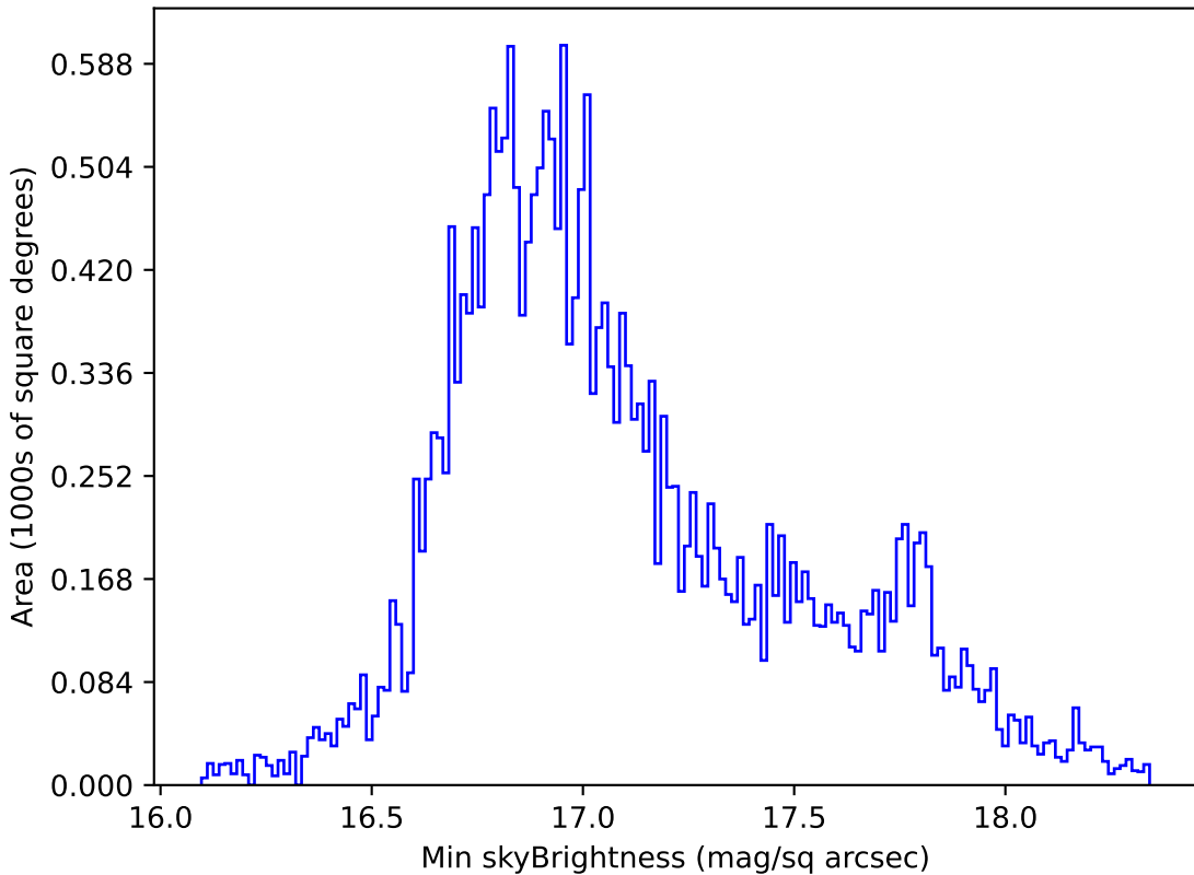
ddf_loaded_fl15_v3.4_10yrs All sky all bands: Min skyBrightness
