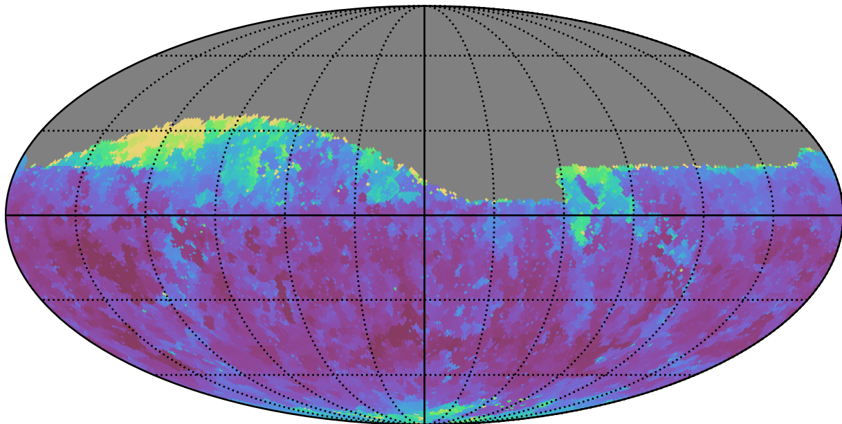
ddf_loaded_fl15_v3.4_10yrs Yr 1 z band: Min seeingGeom
