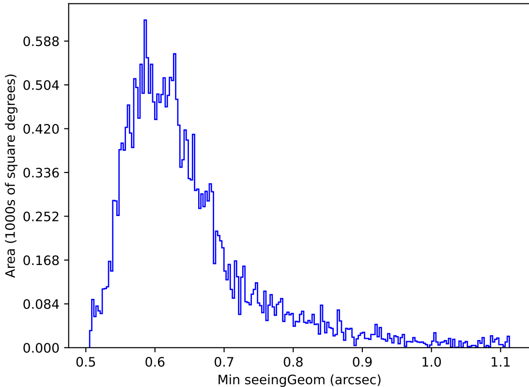
ddf_loaded_fl15_v3.4_10yrs Yr 1 z band: Min seeingGeom
