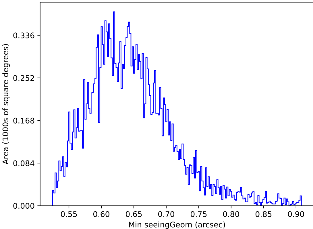
ddf_loaded_fl15_v3.4_10yrs Yr 1 y band: Min seeingGeom
