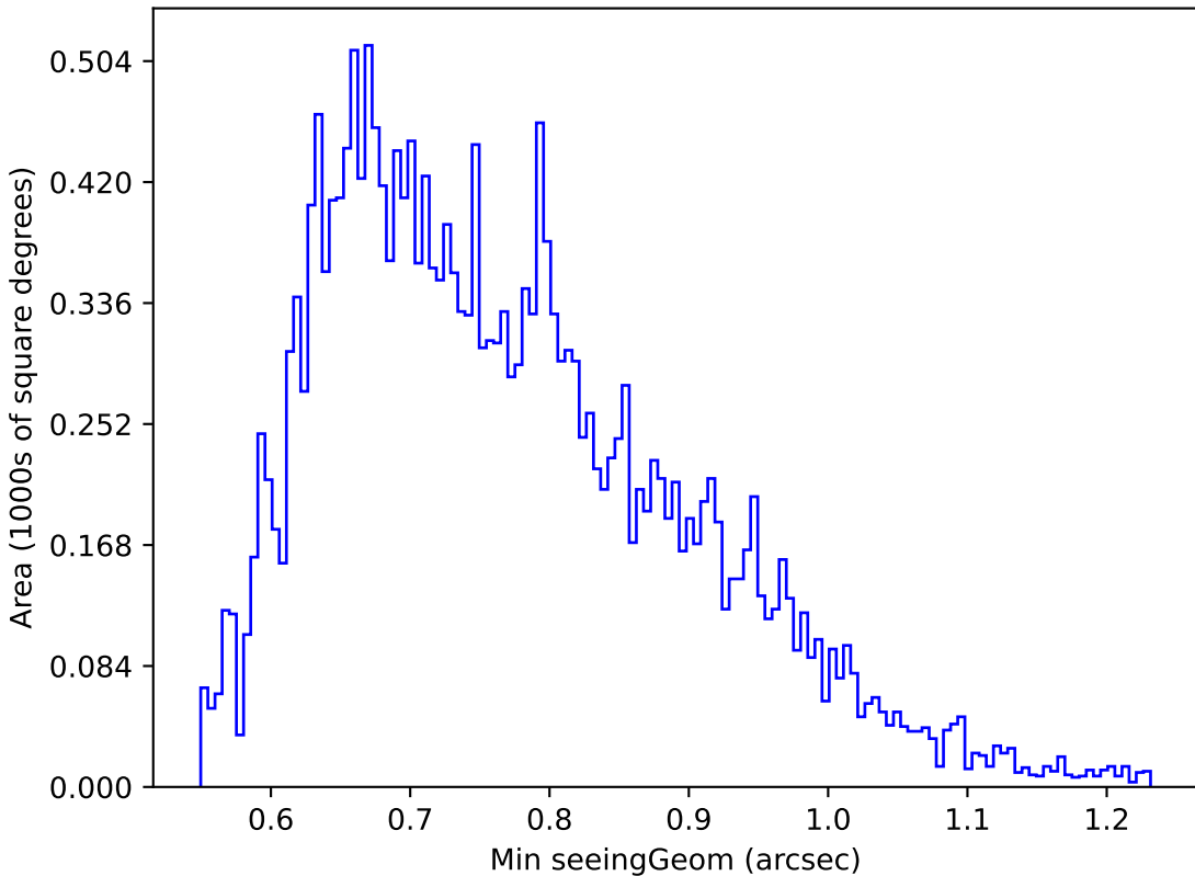
ddf_loaded_fl15_v3.4_10yrs Yr 1 u band: Min seeingGeom
