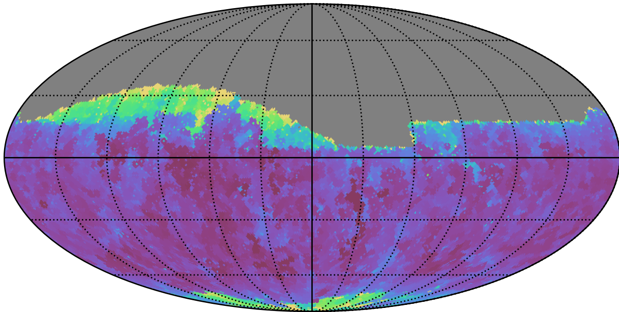
ddf_loaded_fl15_v3.4_10yrs Yr 1 r band: Min seeingGeom
