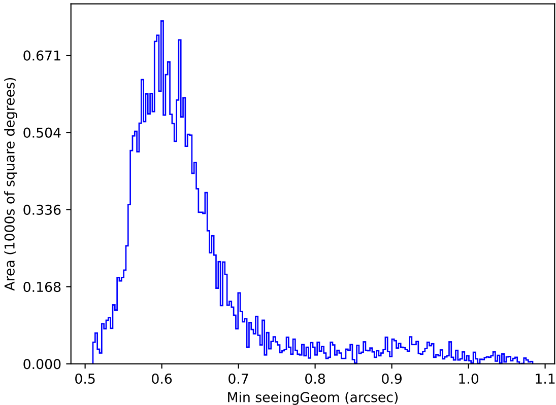
ddf_loaded_fl15_v3.4_10yrs Yr 1 r band: Min seeingGeom
