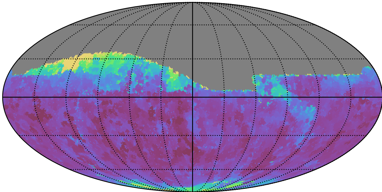
ddf_loaded_fl15_v3.4_10yrs Yr 1 i band: Min seeingGeom
