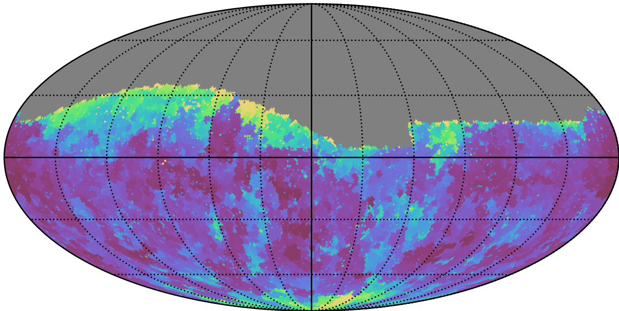
ddf_loaded_fl15_v3.4_10yrs Yr 1 g band: Min seeingGeom
