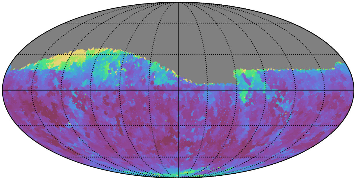
ddf_loaded_fl15_v3.4_10yrs Yr 1 z band: Min seeingEff
