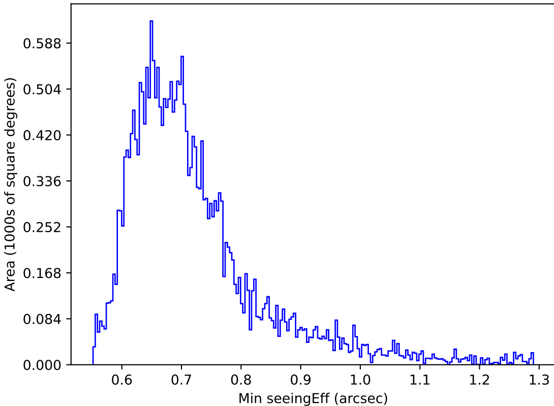
ddf_loaded_fl15_v3.4_10yrs Yr 1 z band: Min seeingEff
