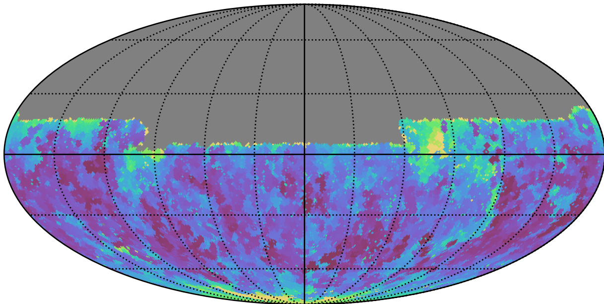
ddf_loaded_fl15_v3.4_10yrs Yr 1 y band: Min seeingEff
