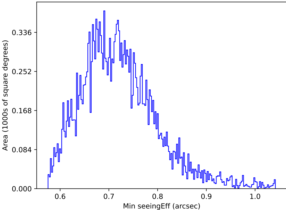
ddf_loaded_fl15_v3.4_10yrs Yr 1 y band: Min seeingEff
