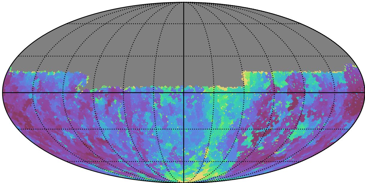
ddf_loaded_fl15_v3.4_10yrs Yr 1 u band: Min seeingEff
