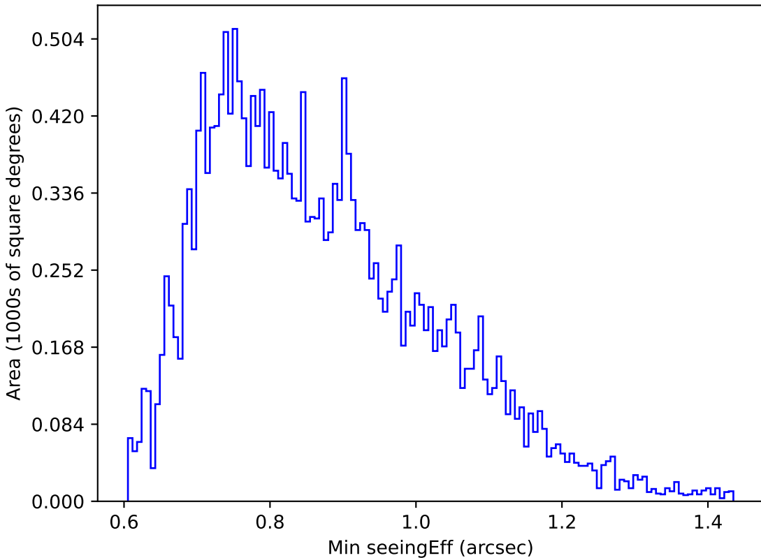
ddf_loaded_fl15_v3.4_10yrs Yr 1 u band: Min seeingEff
