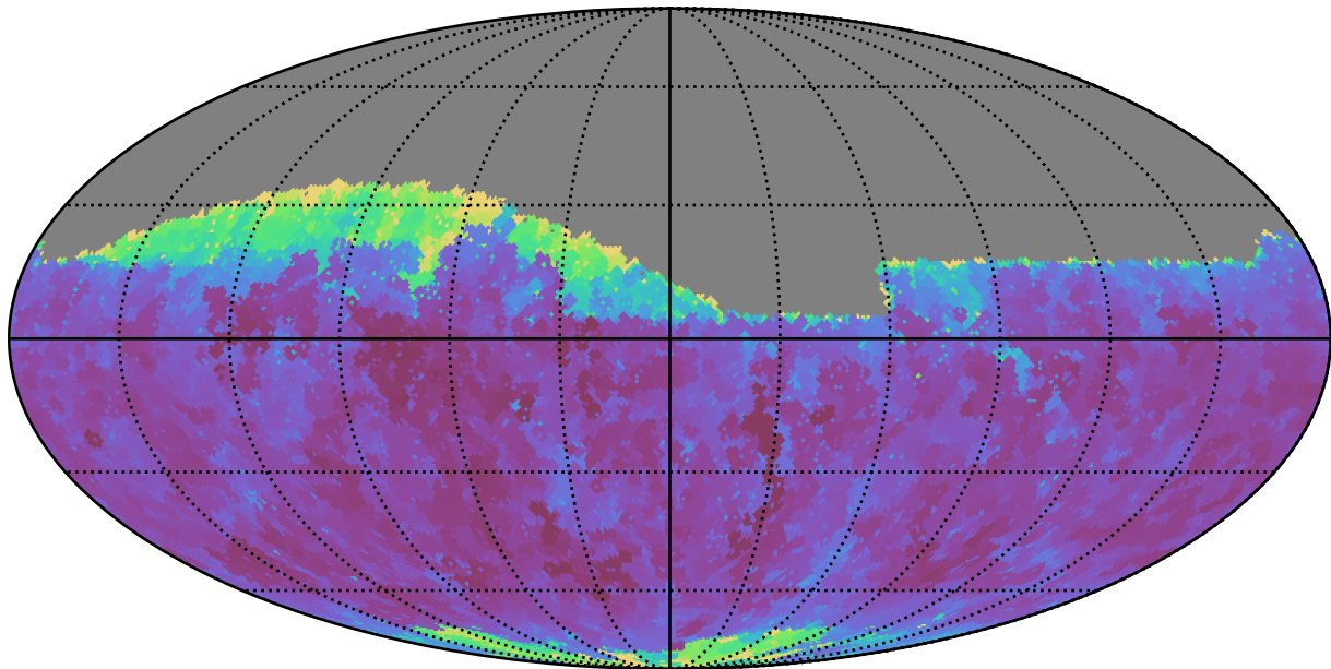
ddf_loaded_fl15_v3.4_10yrs Yr 1 r band: Min seeingEff
