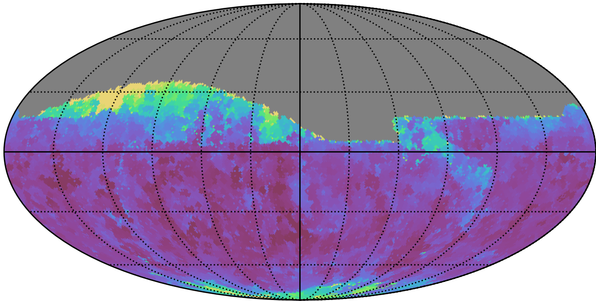
ddf_loaded_fl15_v3.4_10yrs Yr 1 i band: Min seeingEff
