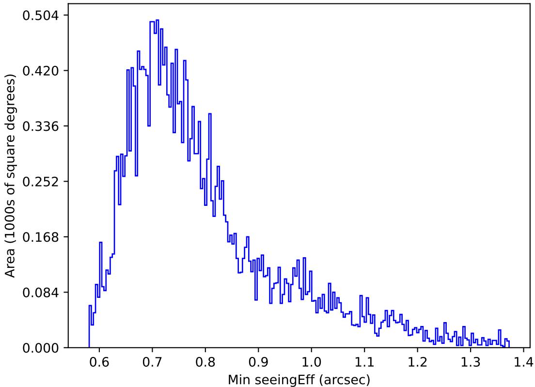
ddf_loaded_fl15_v3.4_10yrs Yr 1 g band: Min seeingEff
