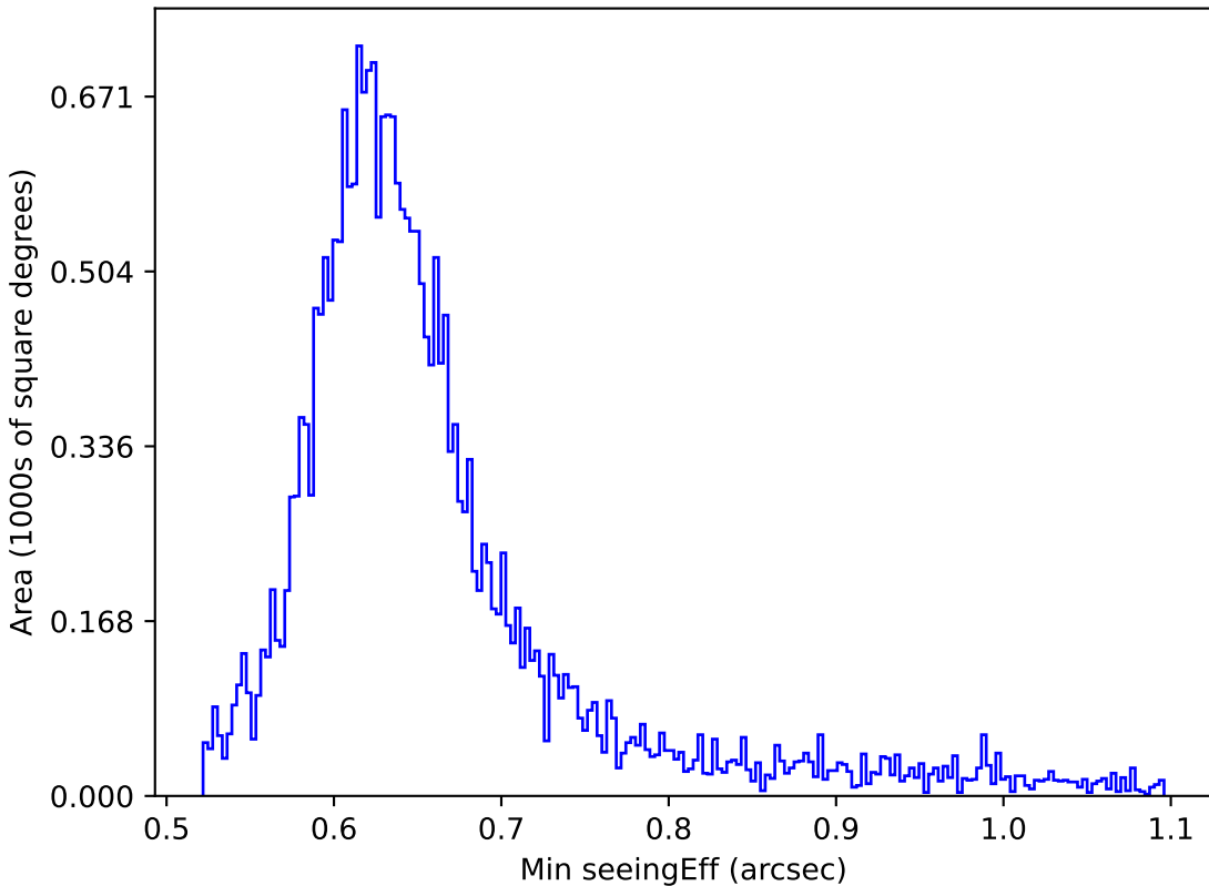
ddf_loaded_fl15_v3.4_10yrs Yr 1 all bands: Min seeingEff
