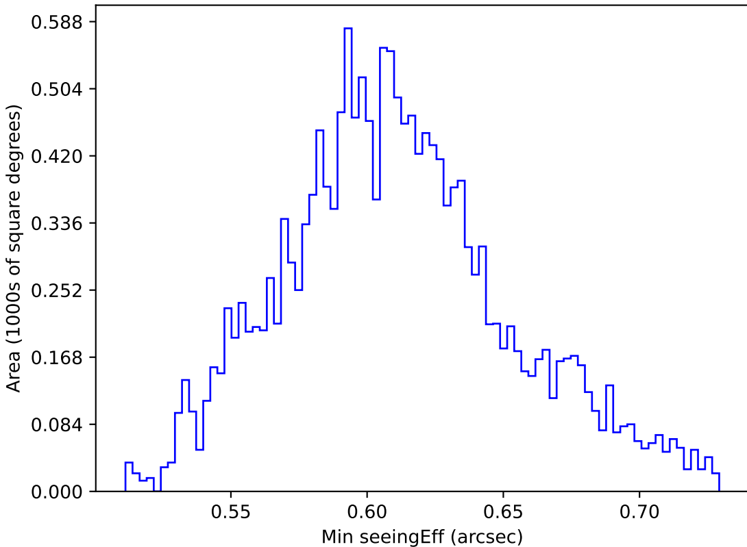
ddf_loaded_fl15_v3.4_10yrs WFD z band: Min seeingEff
