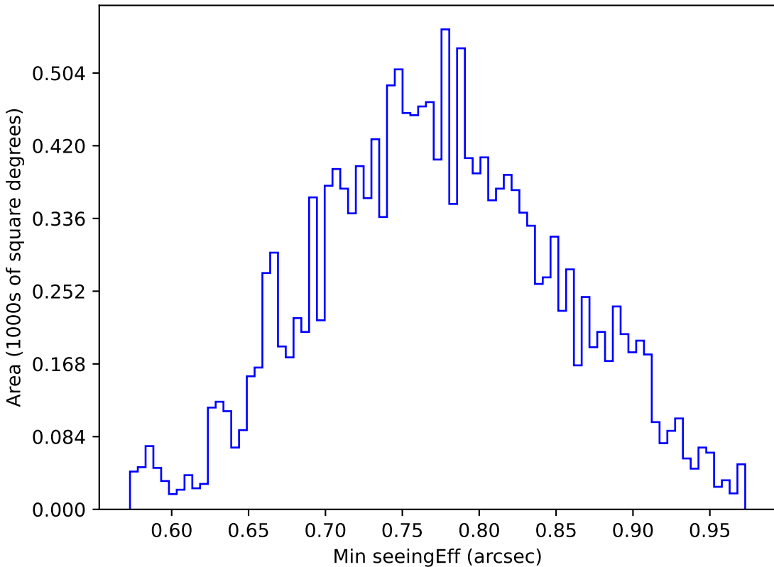
ddf_loaded_fl15_v3.4_10yrs WFD u band: Min seeingEff
