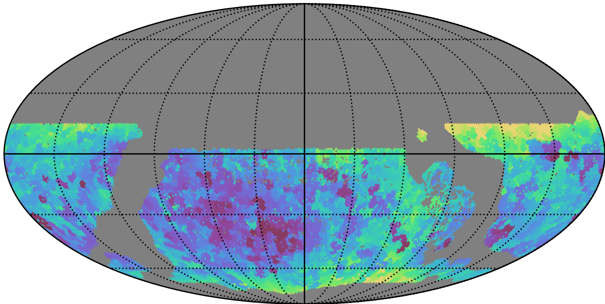
ddf_loaded_fl15_v3.4_10yrs WFD r band: Min seeingEff
