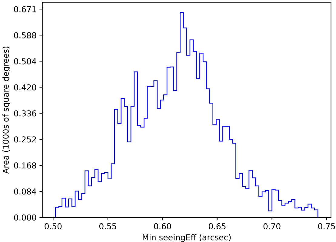
ddf_loaded_fl15_v3.4_10yrs WFD r band: Min seeingEff
