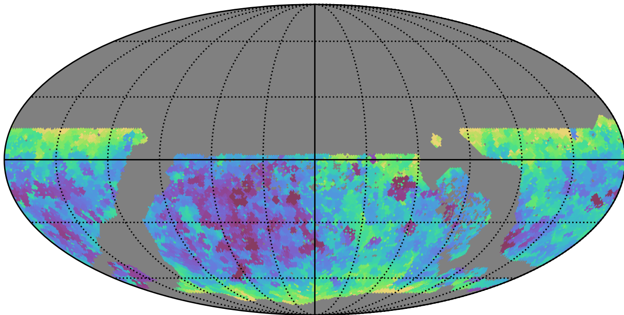
ddf_loaded_fl15_v3.4_10yrs WFD i band: Min seeingEff
