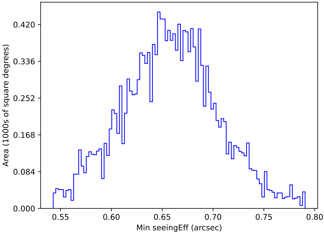
ddf_loaded_fl15_v3.4_10yrs WFD g band: Min seeingEff
