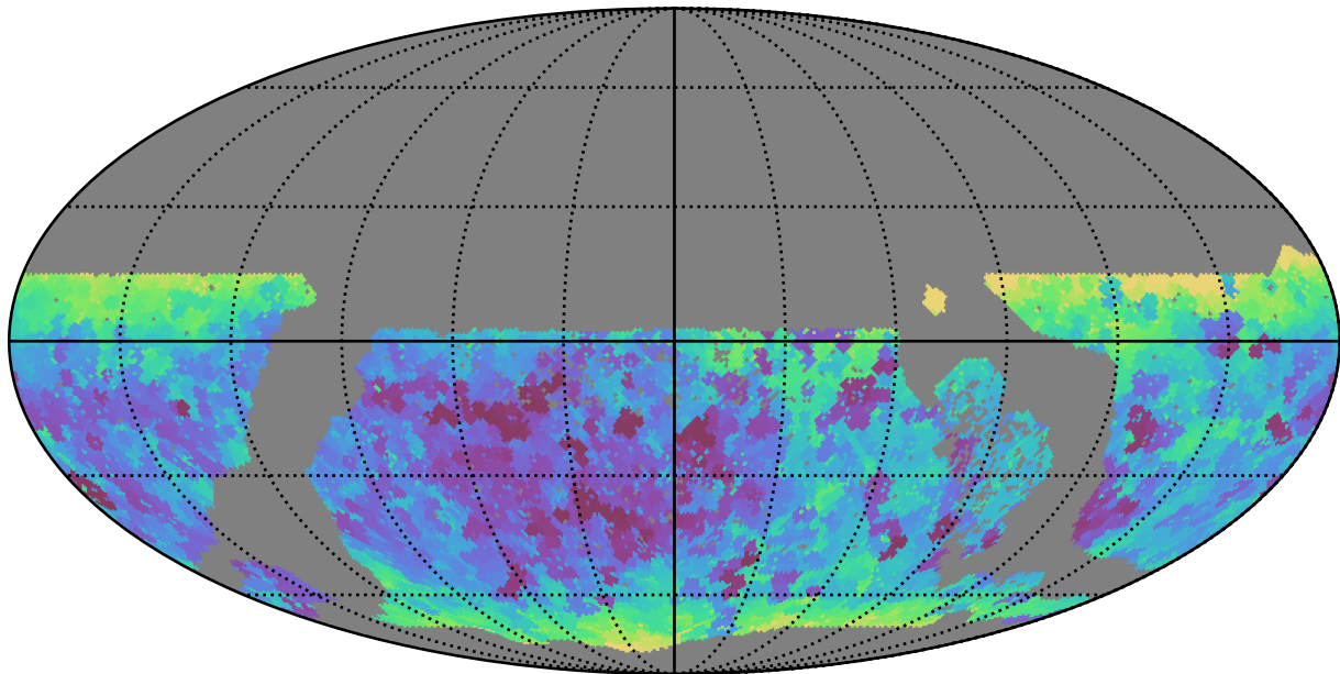
ddf_loaded_fl15_v3.4_10yrs WFD all bands: Min seeingEff
