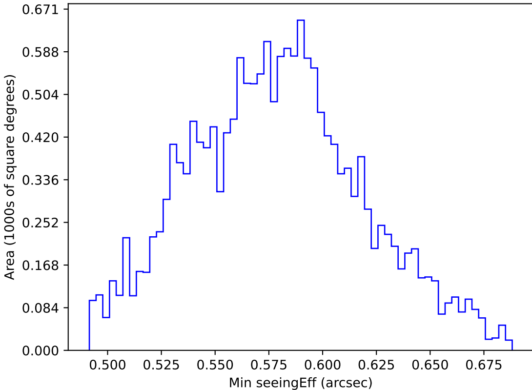
ddf_loaded_fl15_v3.4_10yrs WFD all bands: Min seeingEff
