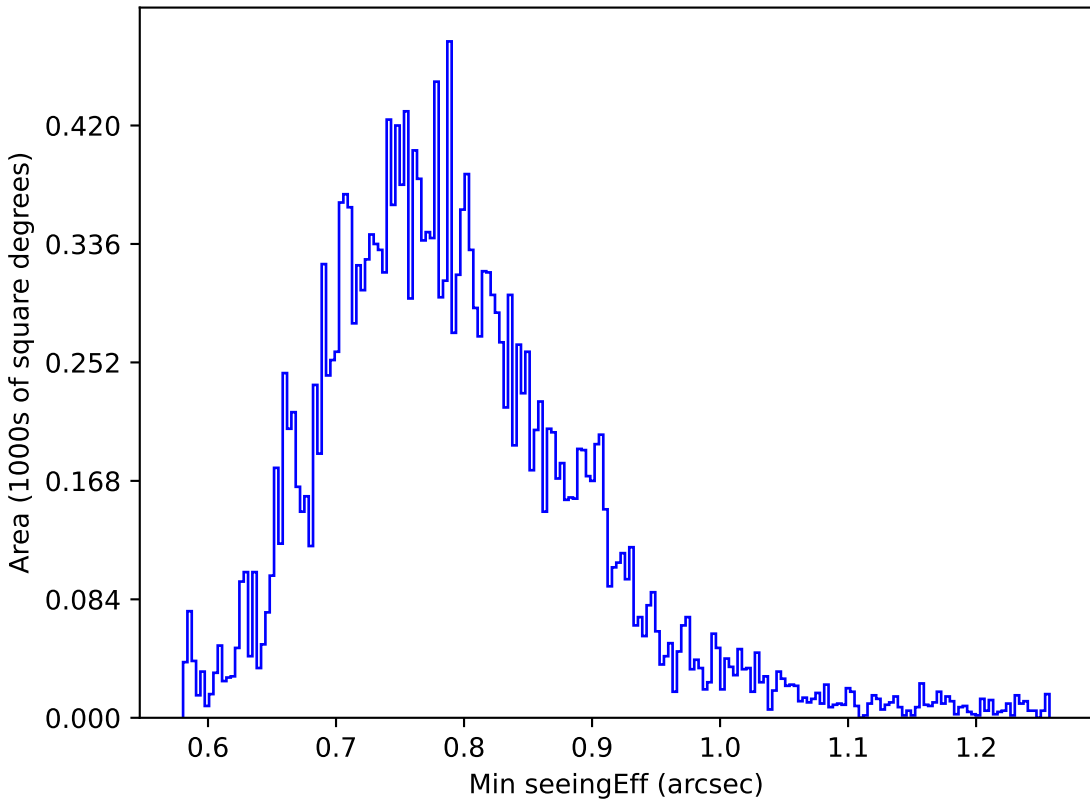
ddf_loaded_fl15_v3.4_10yrs All sky u band: Min seeingEff
