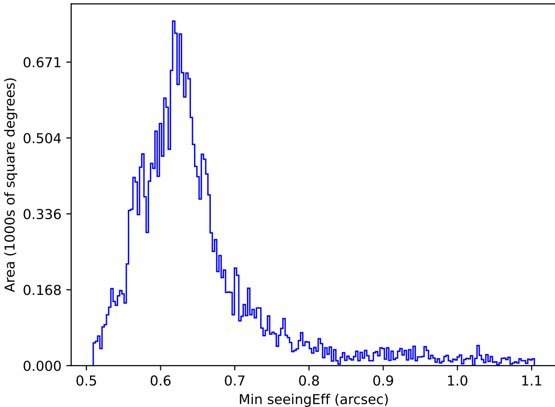
ddf_loaded_fl15_v3.4_10yrs All sky r band: Min seeingEff
